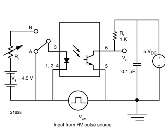
Fig. 3 - Test Circuit for Common Mode Transient Immunity
