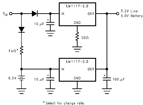
Figure 26. Battery Backed-Up Regulated Supply
