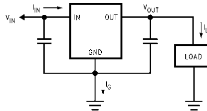
Figure 13. Power Dissipation Diagram
