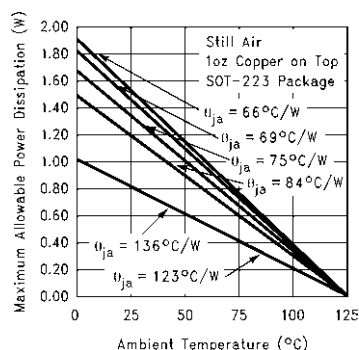
Figure 16. Maximum Allowable Power Dissipation vs. Ambient Temperature for SOT-223
